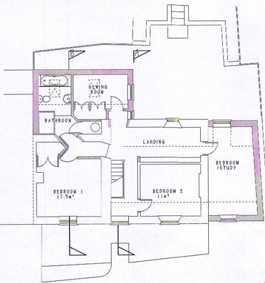
FIRST FLOOR PLAN (new walls shown shaded)
