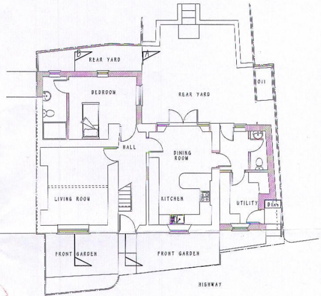
GROUND FLOOR PLAN (new walls shown shaded)
